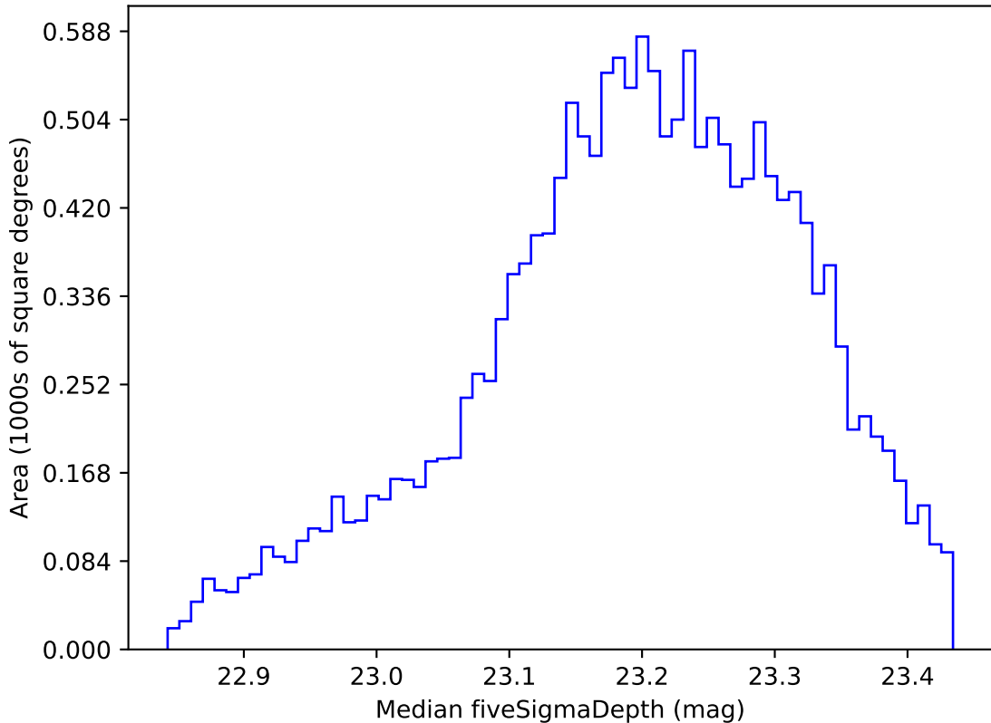
roll_uniform_early_half_mjdp0_v3.4_10yrs WFD u band: Median fiveSigmaDepth
