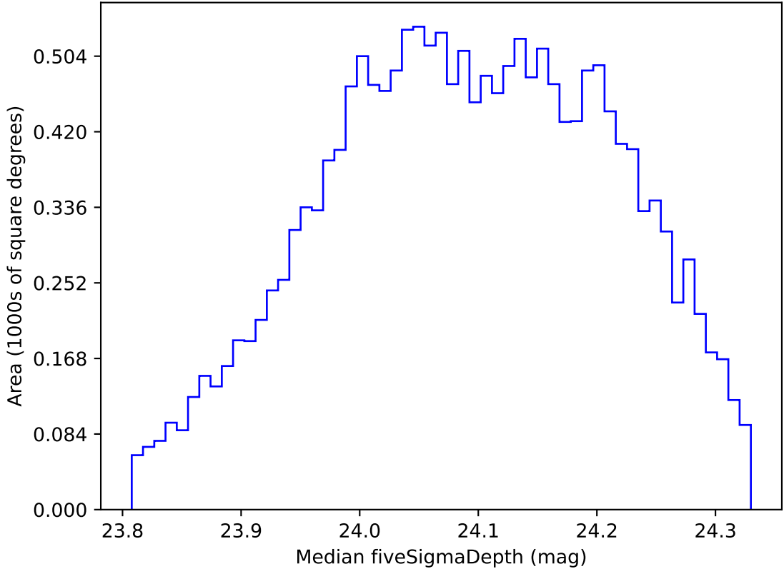
roll_uniform_early_half_mjdp0_v3.4_10yrs WFD r band: Median fiveSigmaDepth
