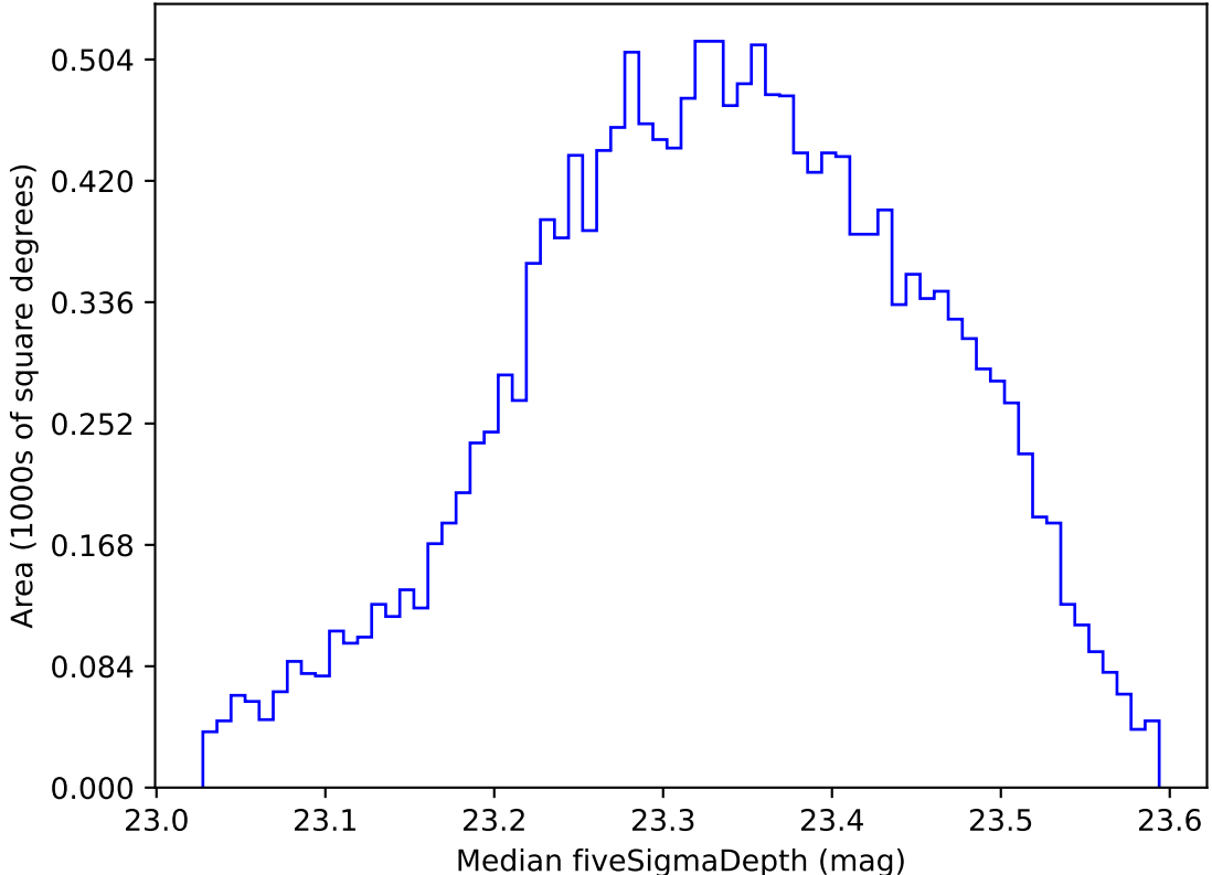
roll_uniform_early_half_mjdp0_v3.4_10yrs WFD all bands: Median fiveSigmaDepth
