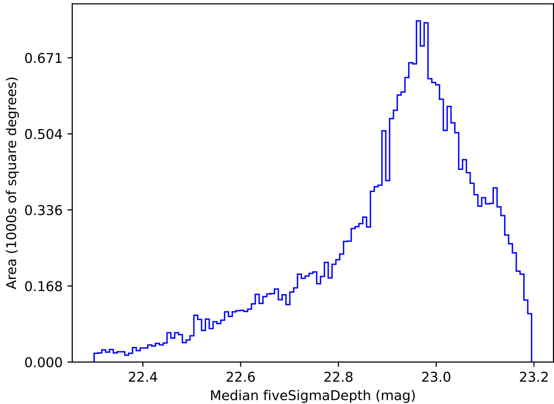
roll_uniform_early_half_mjdp0_v3.4_10yrs All sky z band: Median fiveSigmaDepth
