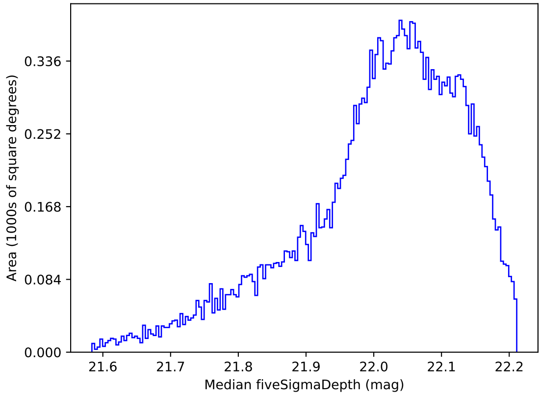
roll_uniform_early_half_mjdp0_v3.4_10yrs All sky y band: Median fiveSigmaDepth
