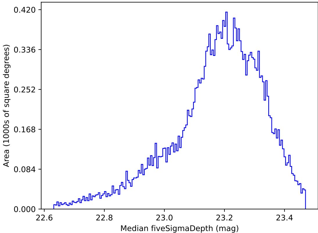
roll_uniform_early_half_mjdp0_v3.4_10yrs All sky u band: Median fiveSigmaDepth
