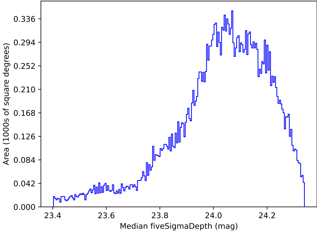
roll_uniform_early_half_mjdp0_v3.4_10yrs All sky r band: Median fiveSigmaDepth
