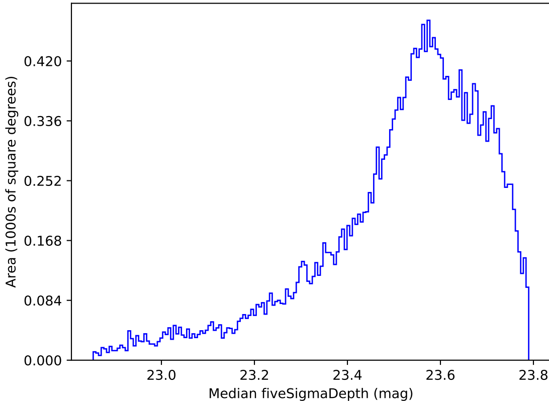
roll_uniform_early_half_mjdp0_v3.4_10yrs All sky i band: Median fiveSigmaDepth
