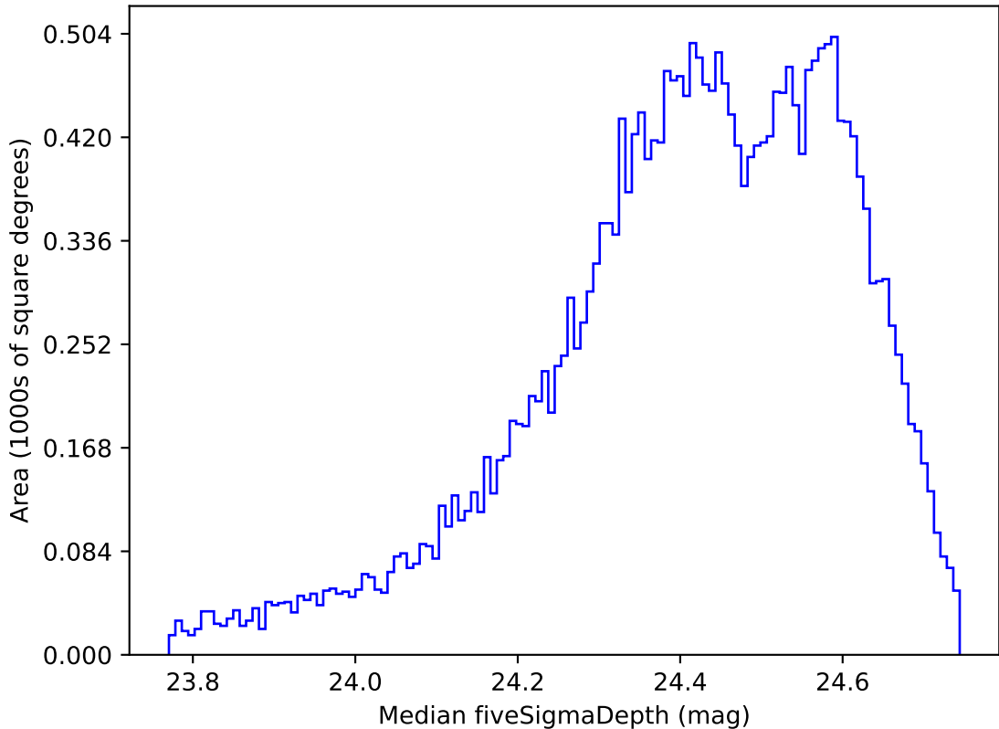
roll_uniform_early_half_mjdp0_v3.4_10yrs All sky g band: Median fiveSigmaDepth
