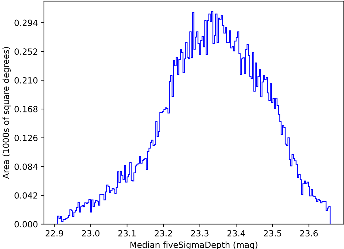
roll_uniform_early_half_mjdp0_v3.4_10yrs All sky all bands: Median fiveSigmaDepth
