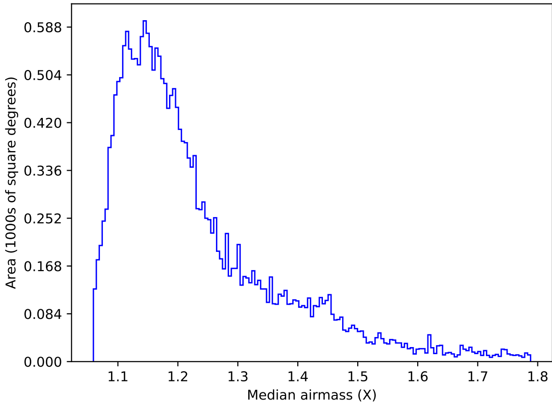
roll_uniform_early_half_mjdp0_v3.4_10yrs Yr 1 u band: Median airmass
