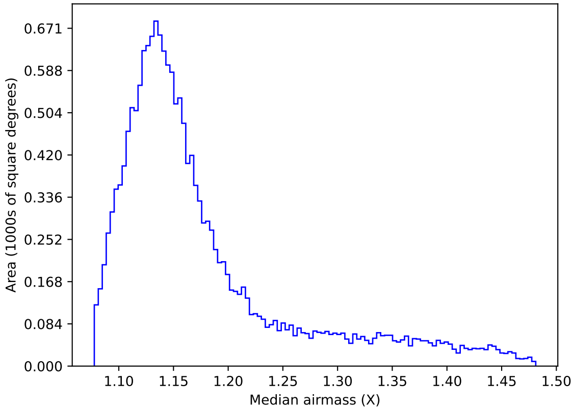
roll_uniform_early_half_mjdp0_v3.4_10yrs WFD g band: Median airmass
