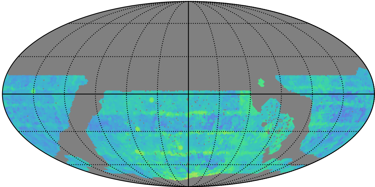
roll_uniform_early_half_mjdp0_v3.4_10yrs WFD z band: Median Season Length
