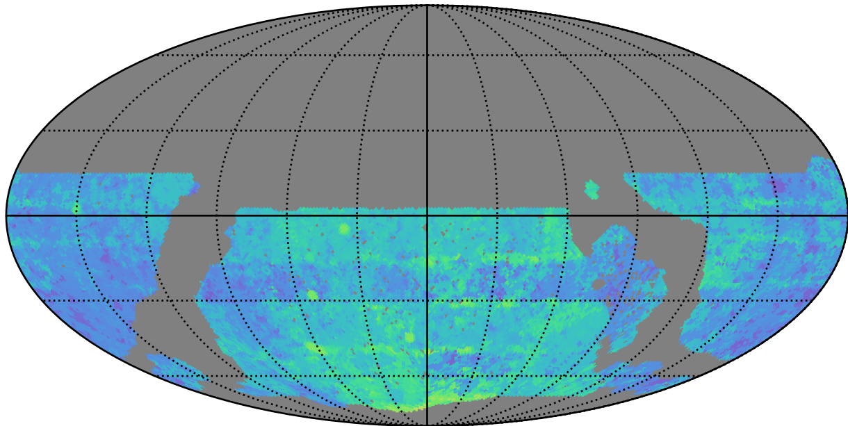
roll_uniform_early_half_mjdp0_v3.4_10yrs WFD y band: Median Season Length
