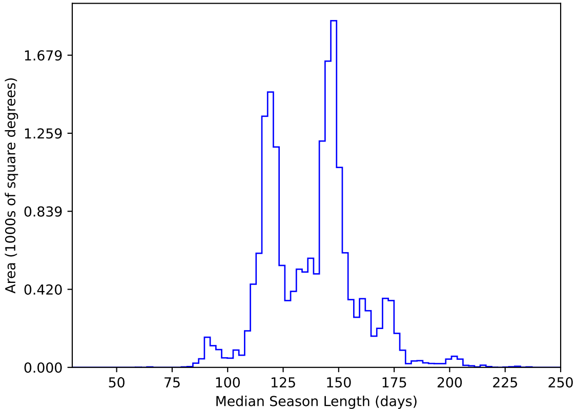
roll_uniform_early_half_mjdp0_v3.4_10yrs WFD y band: Median Season Length
