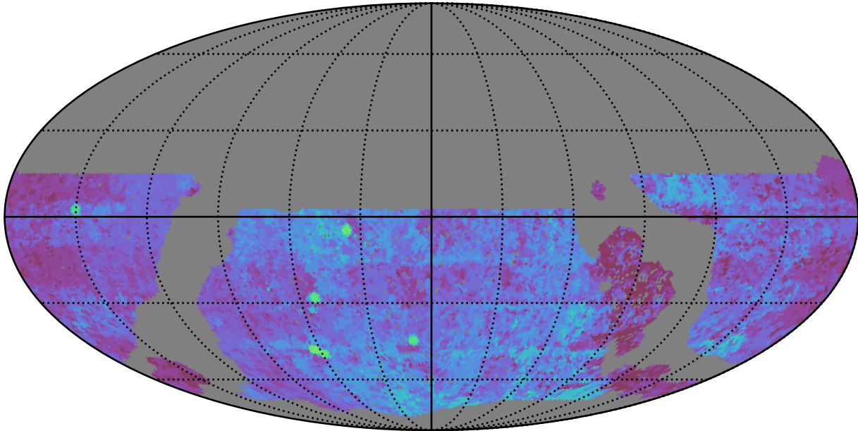
roll_uniform_early_half_mjdp0_v3.4_10yrs WFD u band: Median Season Length
