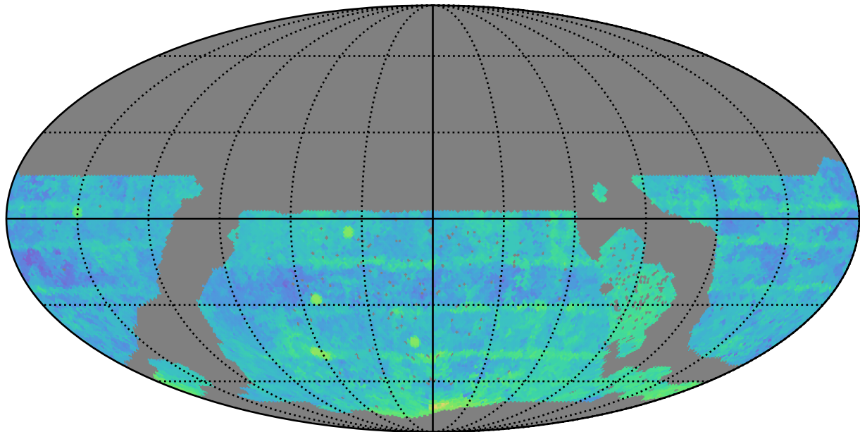
roll_uniform_early_half_mjdp0_v3.4_10yrs WFD r band: Median Season Length
