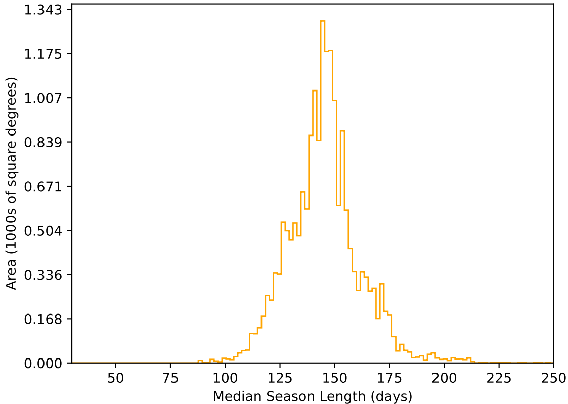
roll_uniform_early_half_mjdp0_v3.4_10yrs WFD r band: Median Season Length
