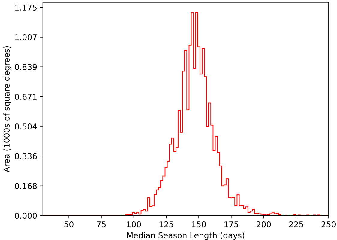
roll_uniform_early_half_mjdp0_v3.4_10yrs WFD i band: Median Season Length
