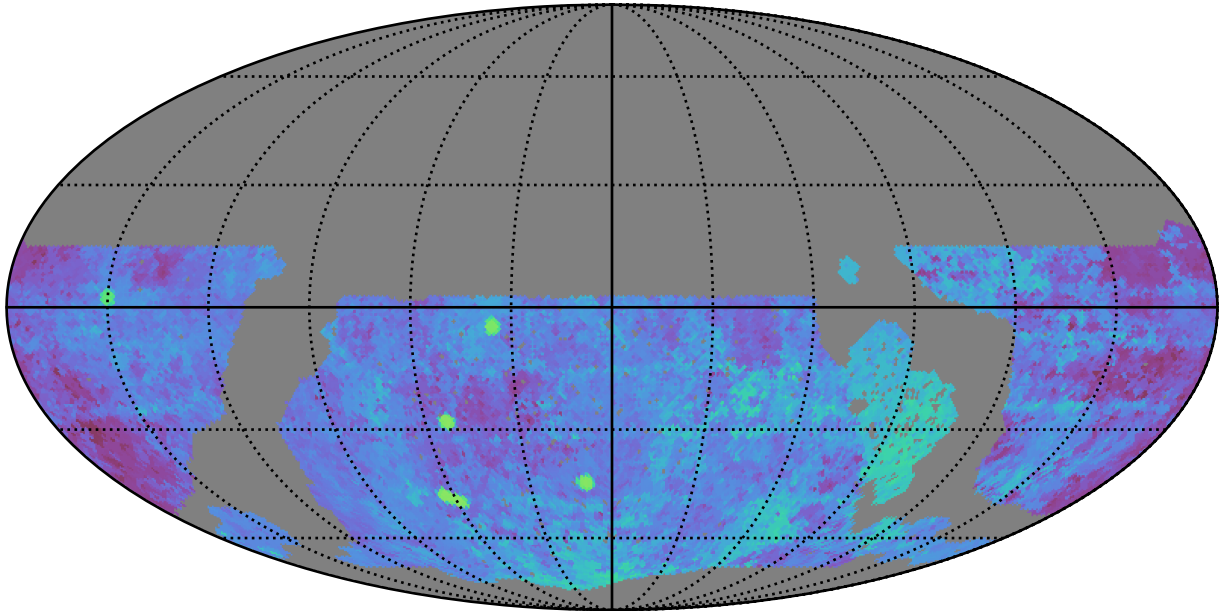
roll_uniform_early_half_mjdp0_v3.4_10yrs WFD g band: Median Season Length
