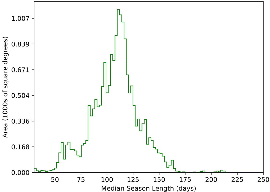
roll_uniform_early_half_mjdp0_v3.4_10yrs WFD g band: Median Season Length
