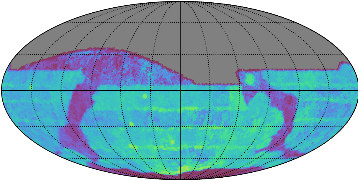
roll_uniform_early_half_mjdp0_v3.4_10yrs All sky z band: Median Season Length
