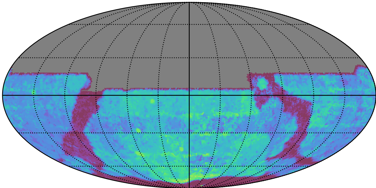
roll_uniform_early_half_mjdp0_v3.4_10yrs All sky y band: Median Season Length
