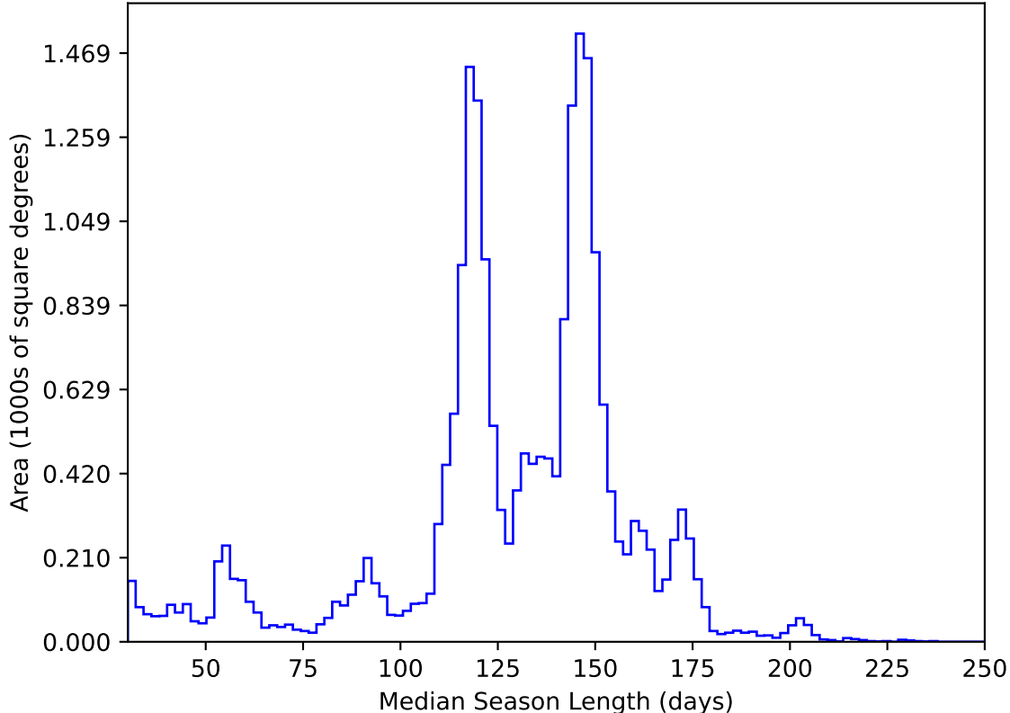
roll_uniform_early_half_mjdp0_v3.4_10yrs All sky y band: Median Season Length
