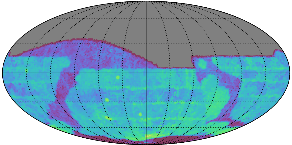
roll_uniform_early_half_mjdp0_v3.4_10yrs All sky r band: Median Season Length
