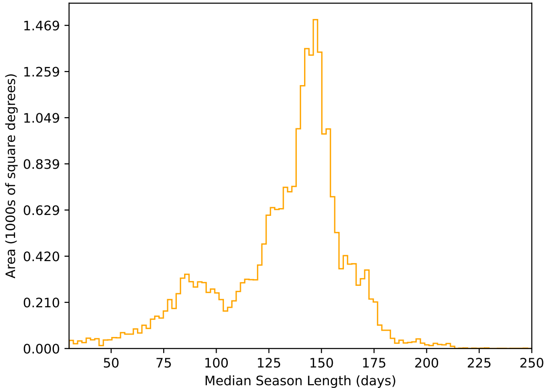
roll_uniform_early_half_mjdp0_v3.4_10yrs All sky r band: Median Season Length
