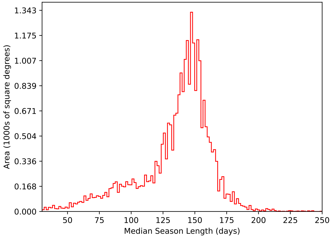
roll_uniform_early_half_mjdp0_v3.4_10yrs All sky i band: Median Season Length
