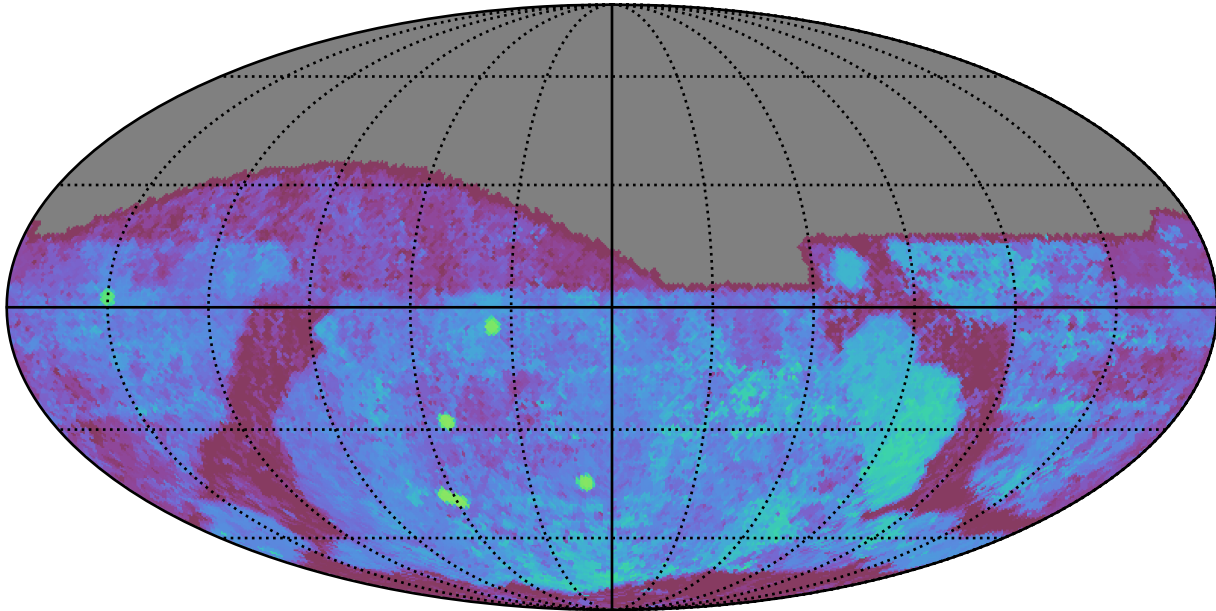
roll_uniform_early_half_mjdp0_v3.4_10yrs All sky g band: Median Season Length
