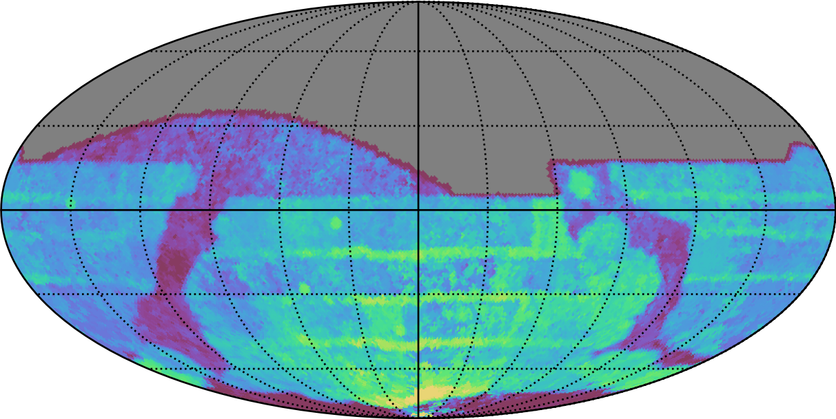
roll_uniform_early_half_mjdp0_v3.4_10yrs All sky all bands: Median Season Length
