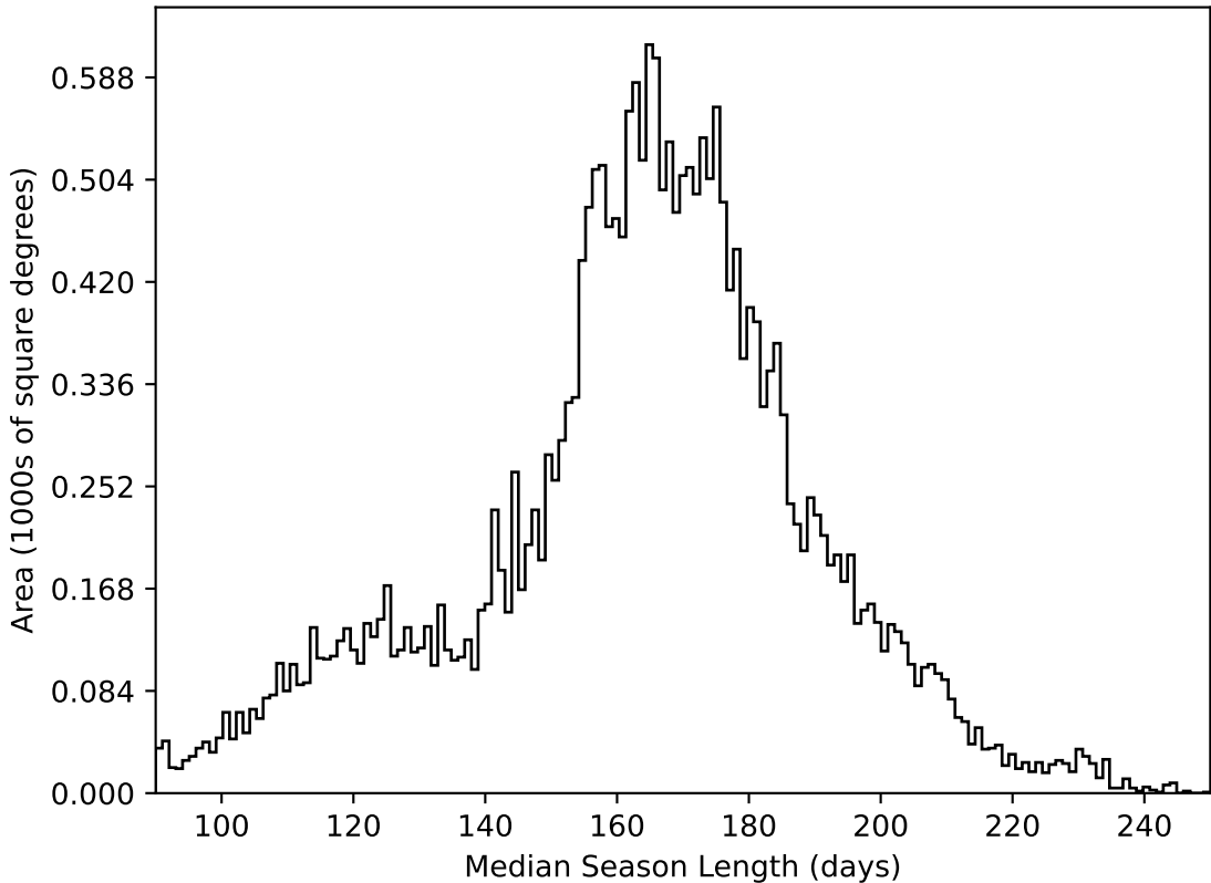
roll_uniform_early_half_mjdp0_v3.4_10yrs All sky all bands: Median Season Length
