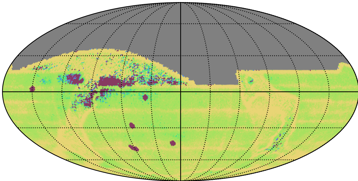
roll_uniform_early_half_mjdp0_v3.4_10yrs All sky: Median Intra-Night Gap
