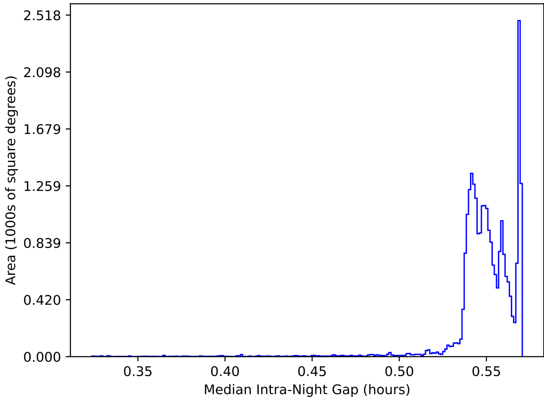
roll_uniform_early_half_mjdp0_v3.4_10yrs All sky: Median Intra-Night Gap
