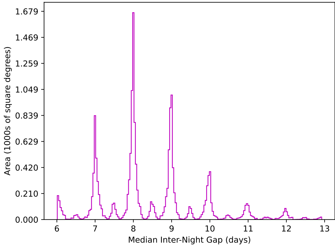
roll_uniform_early_half_mjdp0_v3.4_10yrs WFD z band: Median Inter-Night Gap
