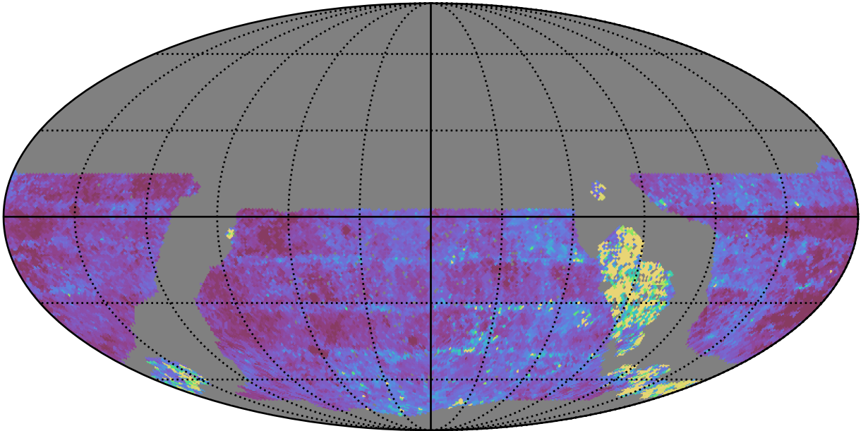
roll_uniform_early_half_mjdp0_v3.4_10yrs WFD u band: Median Inter-Night Gap
