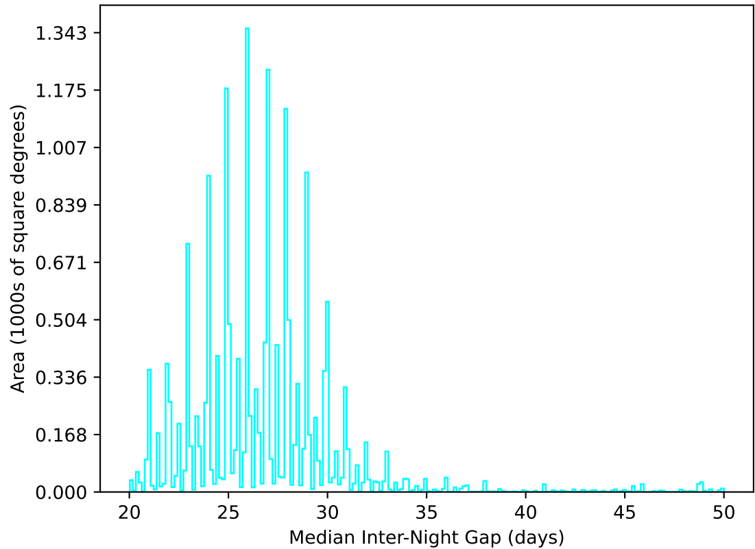
roll_uniform_early_half_mjdp0_v3.4_10yrs WFD u band: Median Inter-Night Gap
