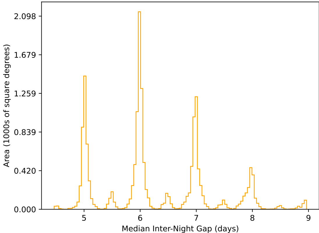
roll_uniform_early_half_mjdp0_v3.4_10yrs WFD r band: Median Inter-Night Gap
