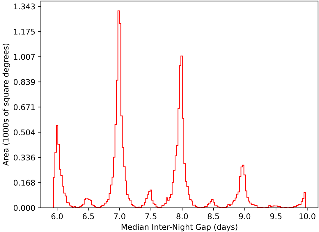
roll_uniform_early_half_mjdp0_v3.4_10yrs WFD i band: Median Inter-Night Gap
