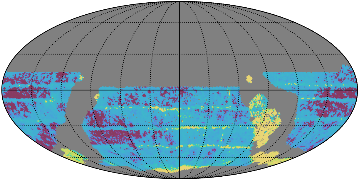
roll_uniform_early_half_mjdp0_v3.4_10yrs WFD all bands: Median Inter-Night Gap
