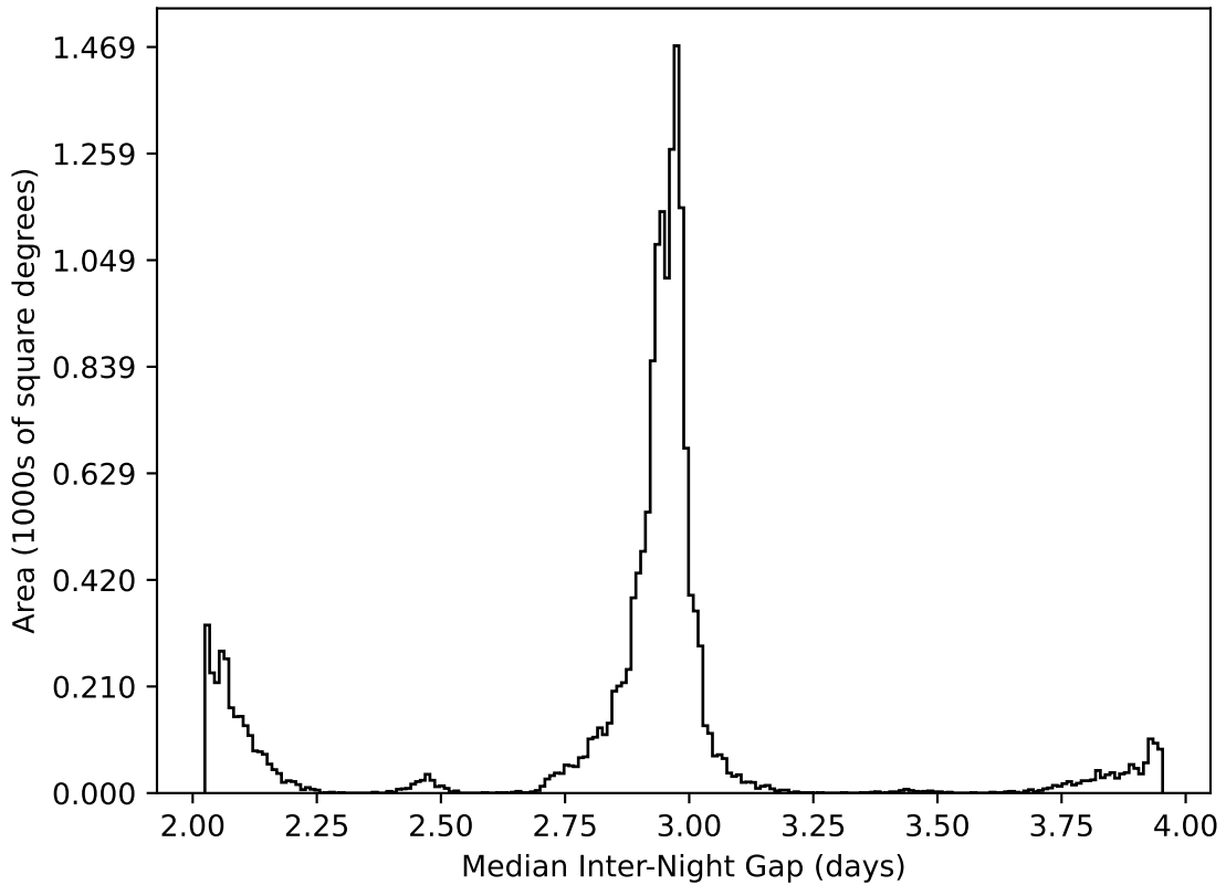
roll_uniform_early_half_mjdp0_v3.4_10yrs WFD all bands: Median Inter-Night Gap
