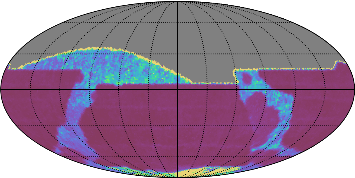
roll_uniform_early_half_mjdp0_v3.4_10yrs All sky z band: Median Inter-Night Gap
