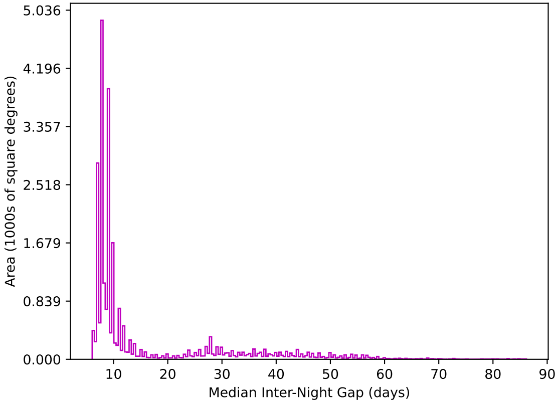
roll_uniform_early_half_mjdp0_v3.4_10yrs All sky z band: Median Inter-Night Gap
