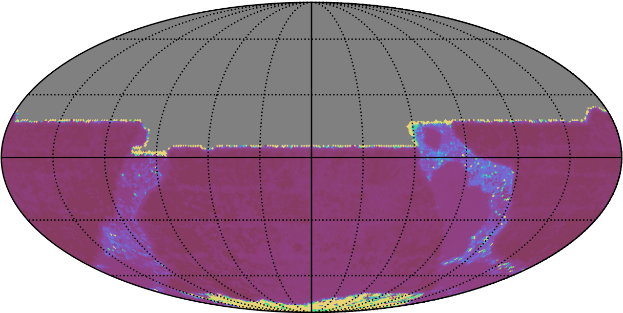
roll_uniform_early_half_mjdp0_v3.4_10yrs All sky y band: Median Inter-Night Gap
