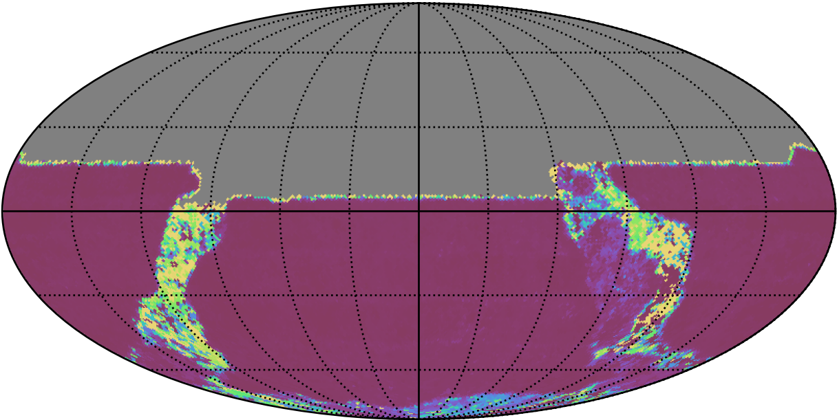
roll_uniform_early_half_mjdp0_v3.4_10yrs All sky u band: Median Inter-Night Gap
