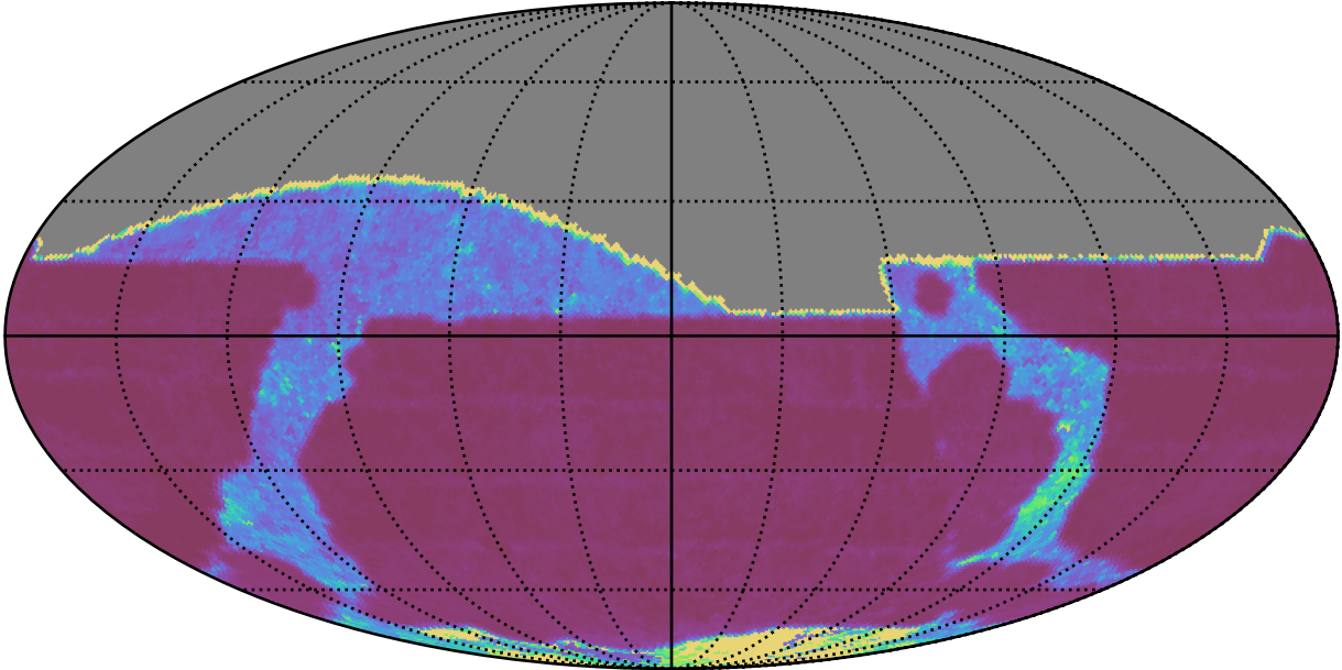
roll_uniform_early_half_mjdp0_v3.4_10yrs All sky r band: Median Inter-Night Gap
