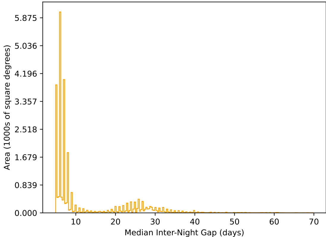
roll_uniform_early_half_mjdp0_v3.4_10yrs All sky r band: Median Inter-Night Gap
