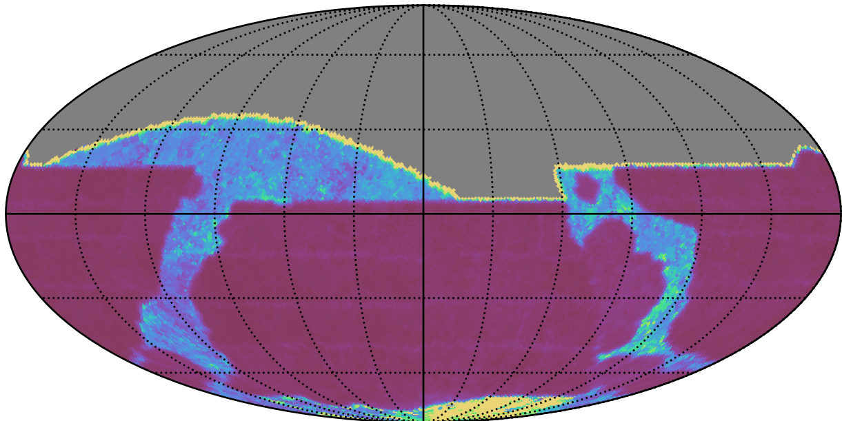
roll_uniform_early_half_mjdp0_v3.4_10yrs All sky i band: Median Inter-Night Gap
