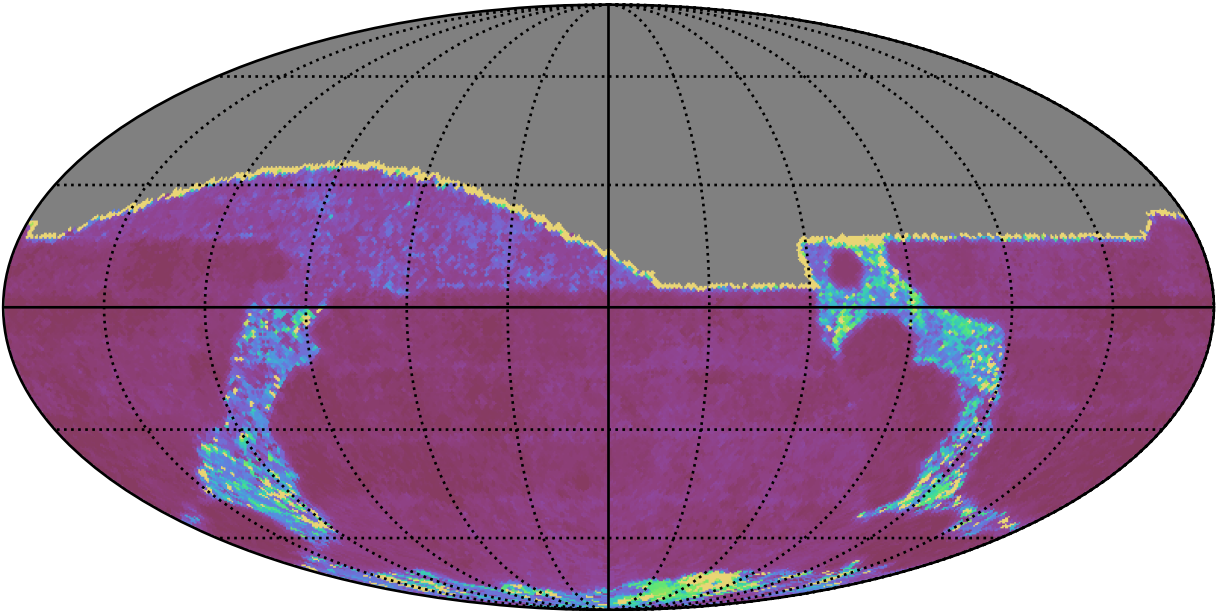
roll_uniform_early_half_mjdp0_v3.4_10yrs All sky g band: Median Inter-Night Gap
