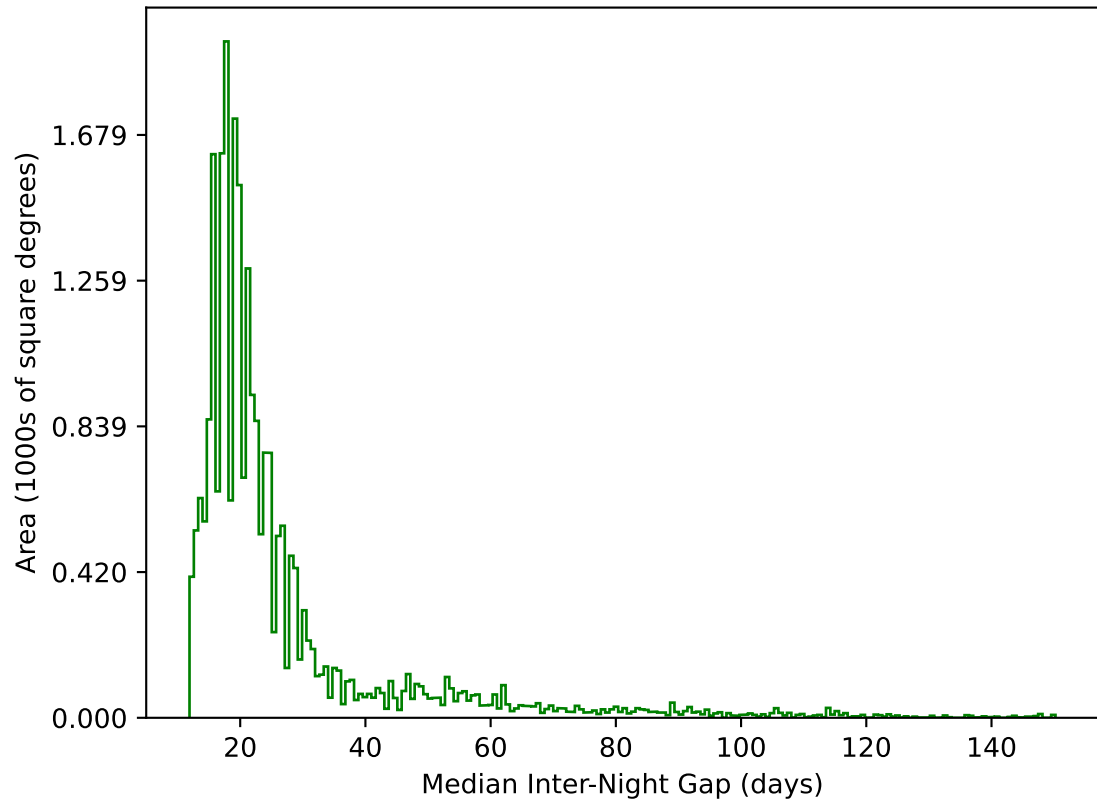
roll_uniform_early_half_mjdp0_v3.4_10yrs All sky g band: Median Inter-Night Gap
