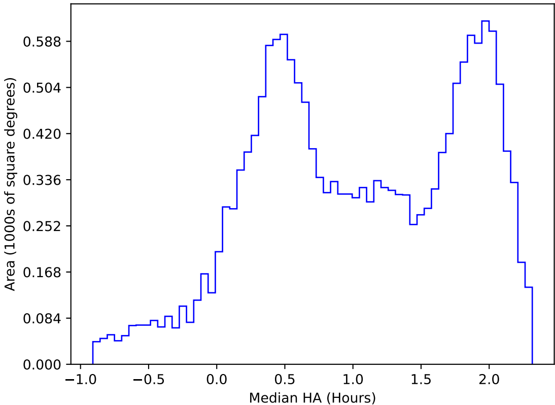
roll_uniform_early_half_mjdp0_v3.4_10yrs WFD z band: Median HA
