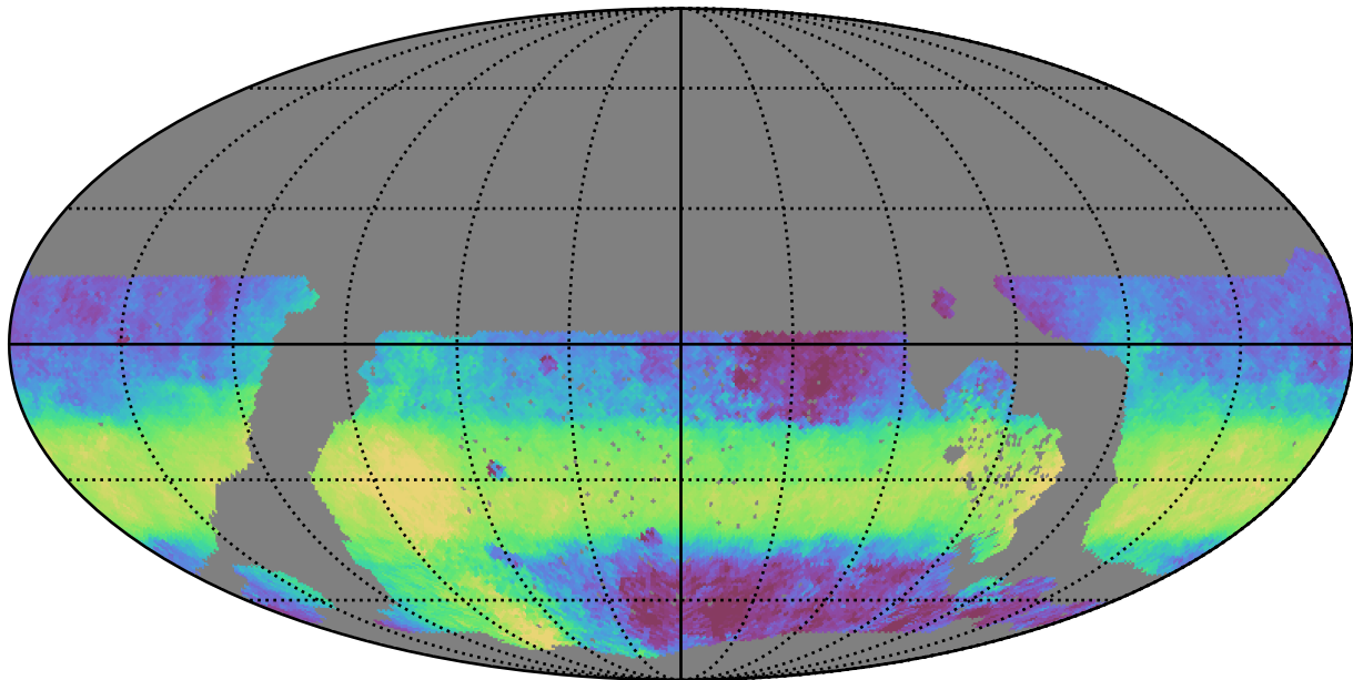
roll_uniform_early_half_mjdp0_v3.4_10yrs WFD y band: Median HA
